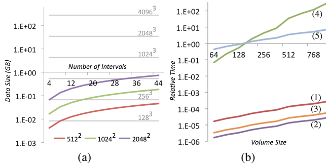
Fig. 15. Cost Evaluation. (a) Space requirements for traditional and proxy-based rendering. We compare storage requirements for volume sizes 128^3 - 4096^3 versus storing k ( k range: 4-44) proxy images of sizes 512^2 , 1024^2 , and 2048^2 . (b) Cost comparison for (1) 3D volume rendering, (2) proxy-based compositing, (3) multi-perspective compositing, (4) 3D ambient occlusion, (5) proxy-based ambient occlusion. This is a pessimistic case, where k is \frac{1}{10} \times volume size and proxy image size is constant ( 512^2 ). Typically, k is constant, as in (a).
