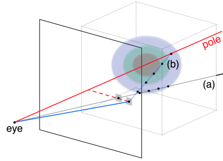
Fig. 5. Volume distortion vs. traditional pinhole camera model. (a) In a traditional pinhole camera, rays are cast from the eye position towards the image plane and into the volume. (b) In our camera, distorted rays are cast from the image plane toward the pole line. We retain the distortion amount and depth as proxy images.
